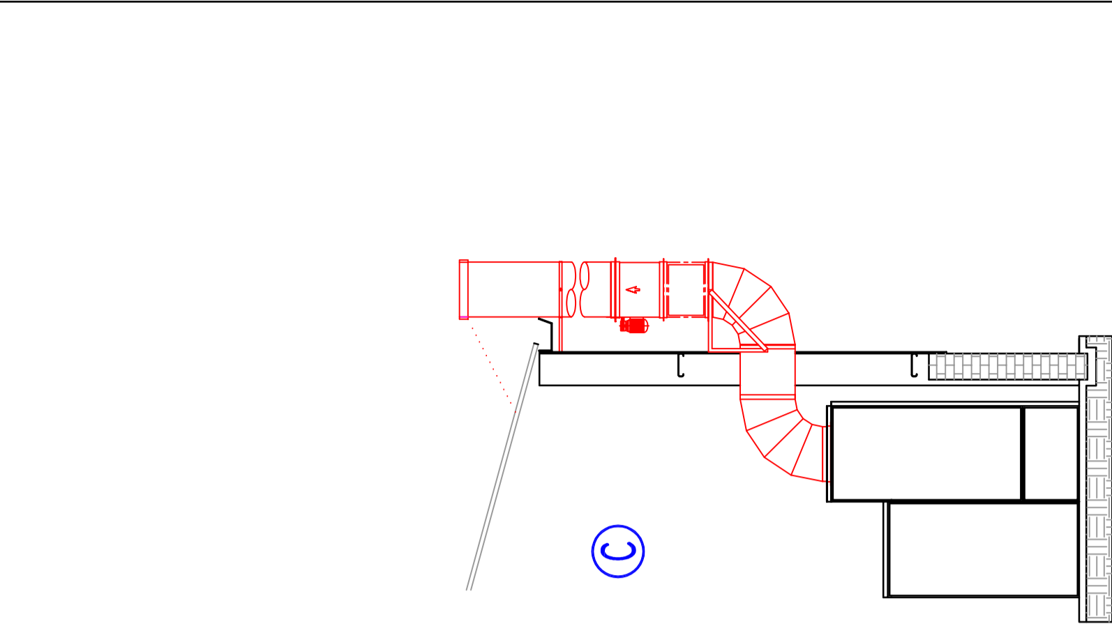
Through-Wall Kit. (High-level external fan)
